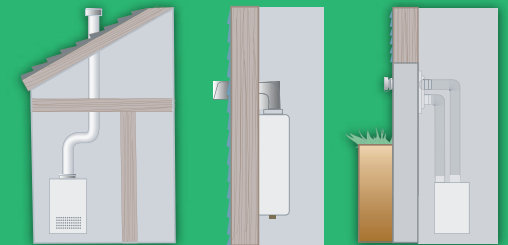
Vertical vent termination
